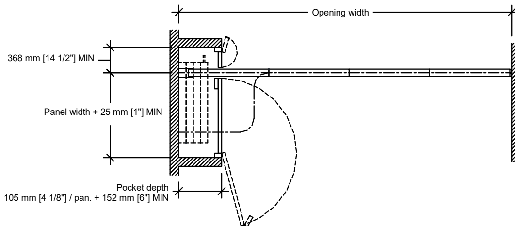
Pocket and PN-3 non-acoustical pocket door (partition seals to back of pocket)
