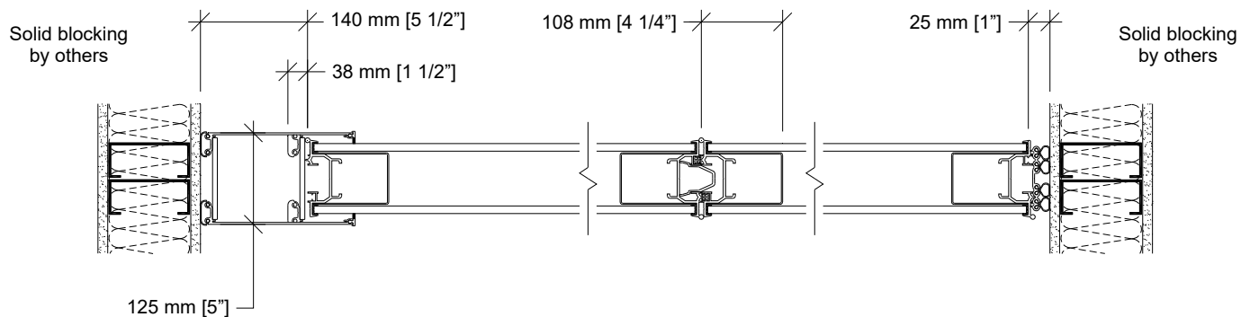
1 Telescopic closure
