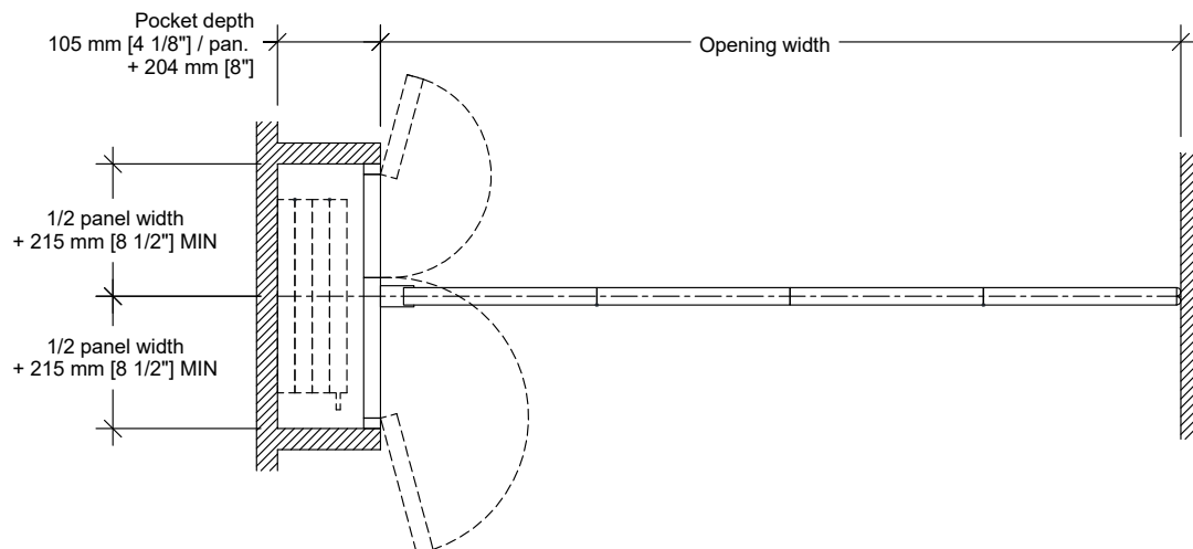
Pocket and PA-82 acoustical pocket door (partition seals to face of pocket door)
