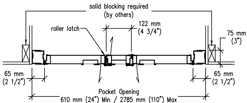
Horizontal Section
