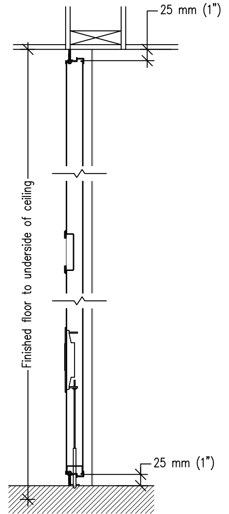
Vertical Section
